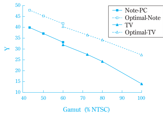
Fig. 6 Gamut vs. Y values of color filters for TV, note-PC and their optimal colors.
