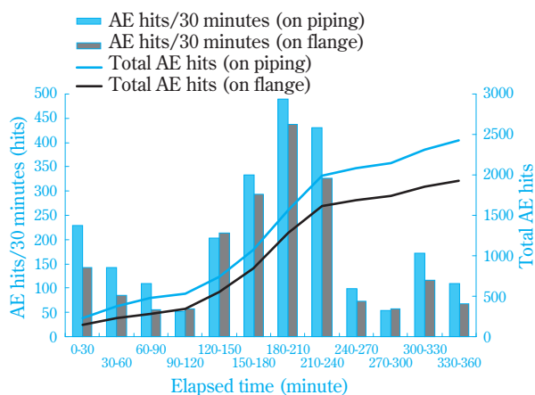
Fig. 15 Comparison of the situation of AE hits piping and flange
