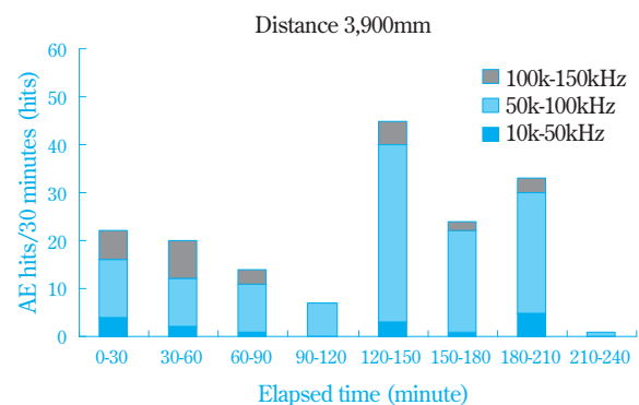
Fig. 12 AE hits by corrosion progress at 3,900mm
