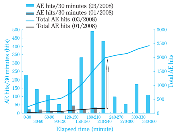
Fig. 16 Comparison of the number of AE hits 01/2008 and 03/2008
