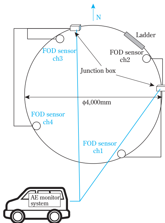
Fig. 18 The position of FOD sensor installation and wiring for signal cable
