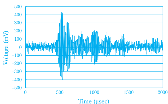
Fig. 24 Representative Waveform of AE obtained before removing rust
