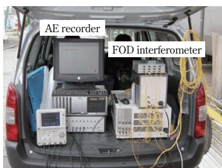
Fig. 21 AE measurement condition in which FOD interferometer and collection analysis device are loaded into car
