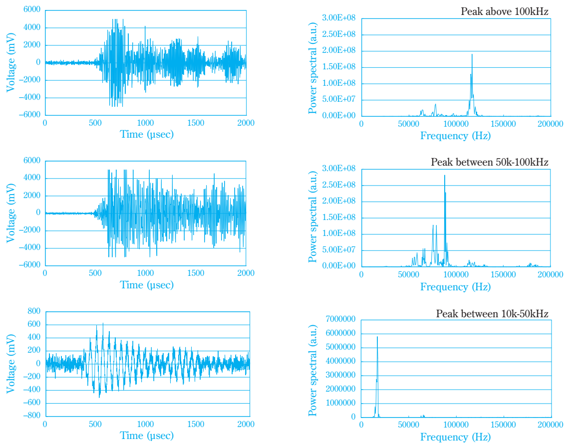
Fig. 10 Data of original AE and Frequency spectrum pattern
