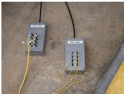
Fig. 20 Connection of 4ch FOD sensor to junk BOX
