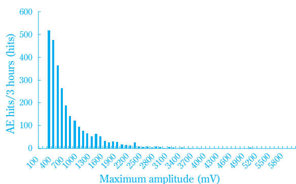
Fig. 29 Distribution of AE hits and maximum amplitude obtained before removing rust
