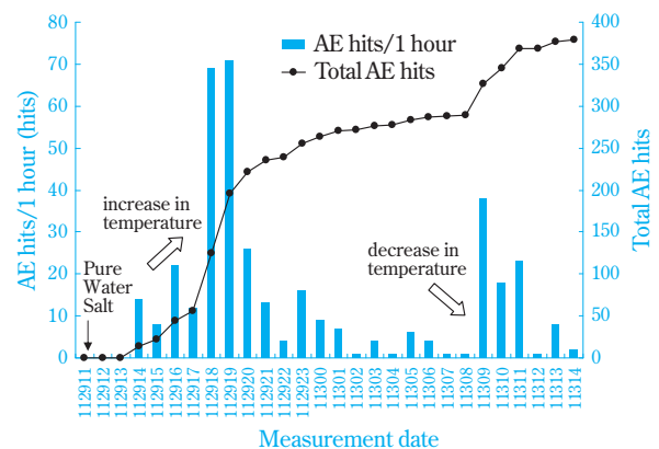
Fig. 9 AE hits by initial corrosion
