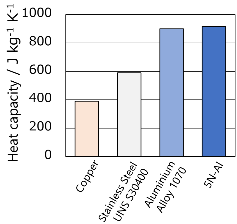
Heat capacity
