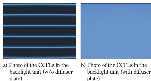
Fig. 3 Basic function of the light diffuser plate (CCFL = Cold Cathode Fluorescent Lamp)
