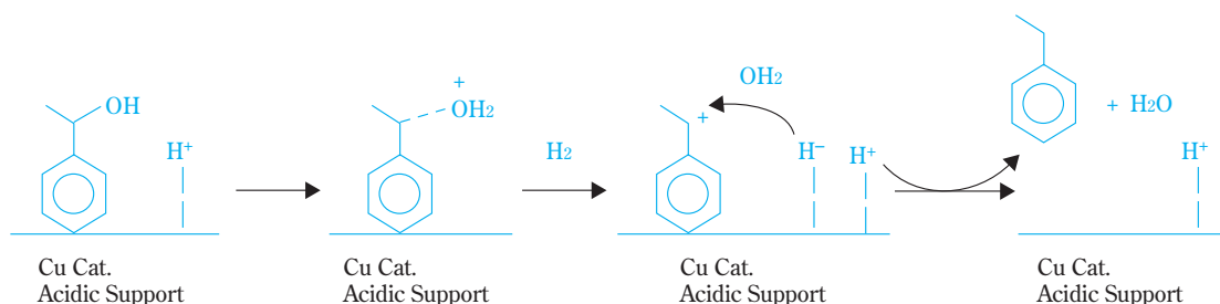
Fig. 4 Scheme of hydrogenolysis of \alpha -phenyl ethanol
