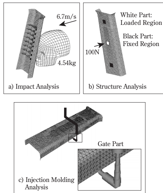
Fig. 21 Simulation Models
