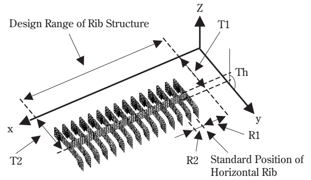
Fig. 11 Design Variables of Rib Structure
