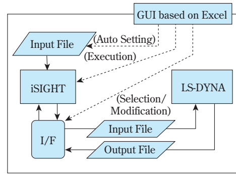
Fig. 22 Schematic Diagram of System
