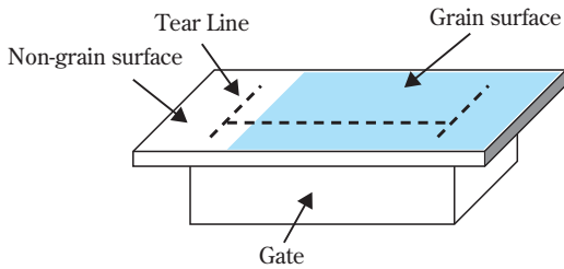
Fig. 13 Overall image of quasi-airbag cover
