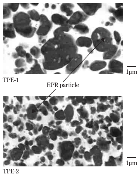
Fig. 9 TEM image of TPEs
