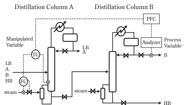
LB : Low Boiling point components HB : High Boiling point components A : component A B : component B FC : Flow rate to be controlled by PID controller TC : Temperature to be controlled by PFC
