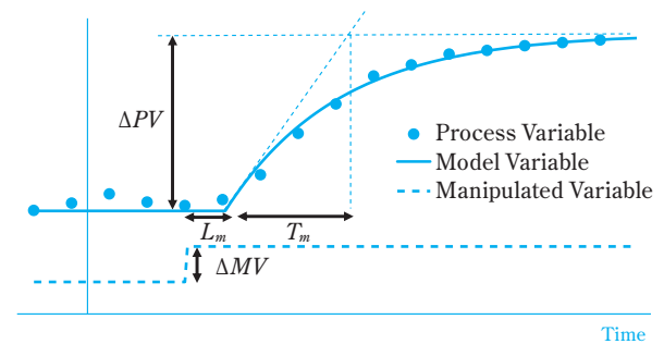
Fig. 7 Actual process response and its approximation by “1 st order + dead time” process model
