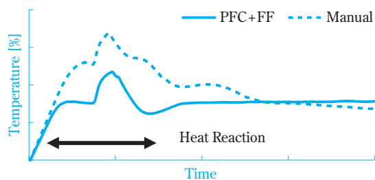
Fig. 17 Comparison of temperature control results by PFC+FF and manual operation
