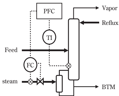
TI : Temperature Indicator FC : Flow Rate to be controlled by PID controller
