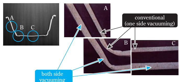
Fig. 7 Cross section of vacuum formed product (noodle bowl)
