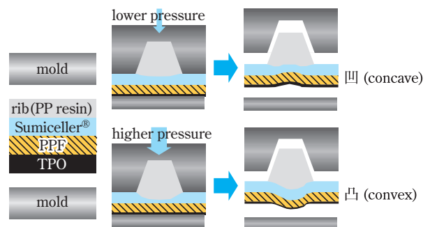
Fig. 5 Unevenness of surface depends on molding pressure
