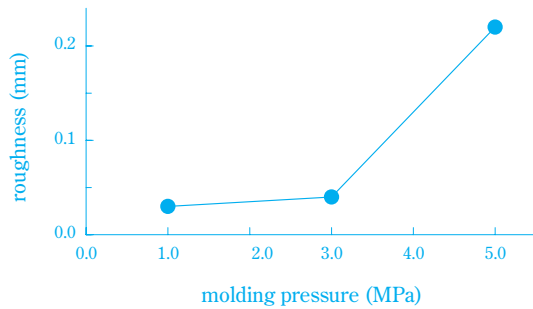
Fig. 6 Roughness (convex) vs. molding pressure
