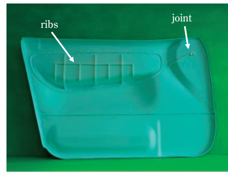
Fig. 4 Back side of door panel by Back Molding Process
