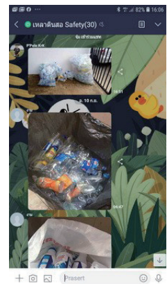
Chat screen
